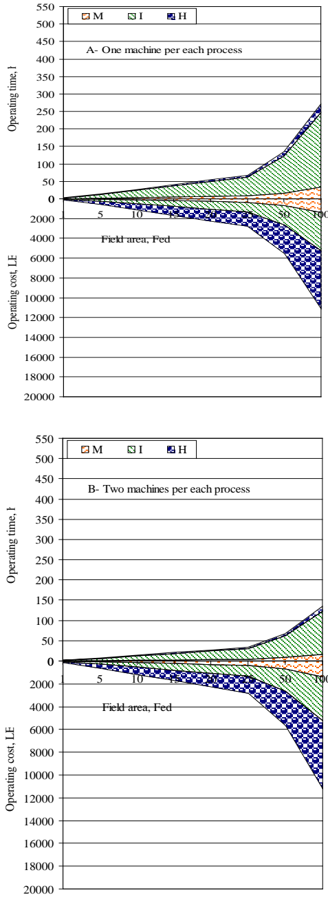
Fig. 10: The accumulative curve for operating time and cost via square field area at (I); (M) and (H) process of 609 m 3 /min discharge and 2.5 and 2.5 m widths respectively.
