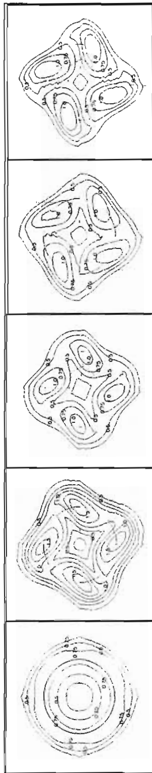
A1) Baseline jet (without inj.) A2) SJ \alpha=0^\circ mr=.055 A3) SJ \alpha=45^\circ mr=.055 A4) SJ \alpha=0^\circ mr=.078 A5) SJ \alpha=45^\circ mr=.078 Fig. 9 Computational iso-contour of turbulence kinetic energy ( k ) for baseline jet and swirl jet at a horizontal plane. Z/D=3 .
