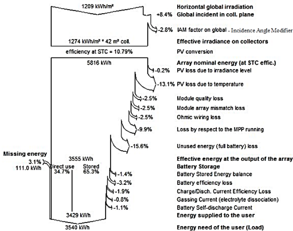
Fig. 9. Loss diagram over the whole year [authors processed by PVSYST]
