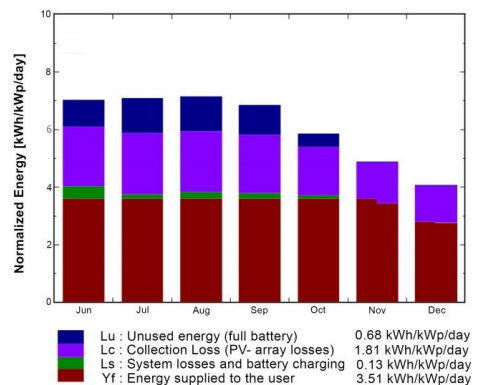
Normalized productions (per installed kWp) : Normal power 4560 Wp
