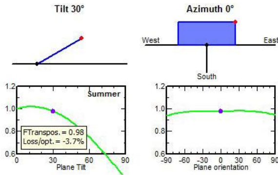
Fig. 7. PV field type: Fixed tilted plane [authors processed by PVSYST]
