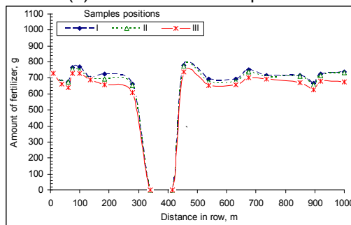
(b) 4.38 km/h forward speed.
