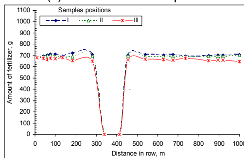
(c) 4.79 km/h forward speed.
