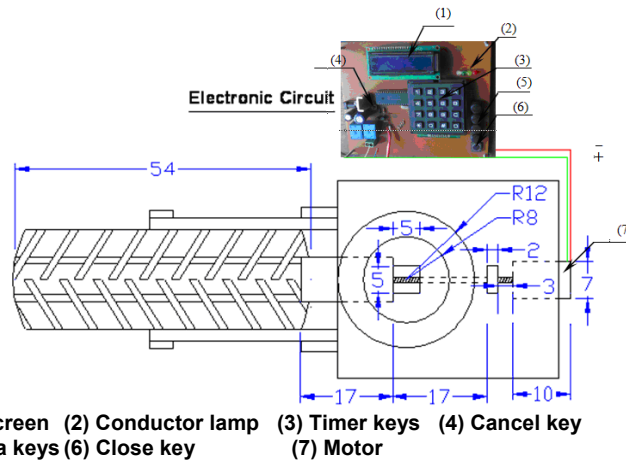
Fig. 5: A schematic diagram of feed gate and electronic elements.
