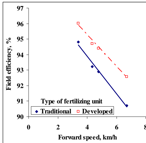
Fig. (8) Effect of forward speeds on field efficiency using fertilizing units.
