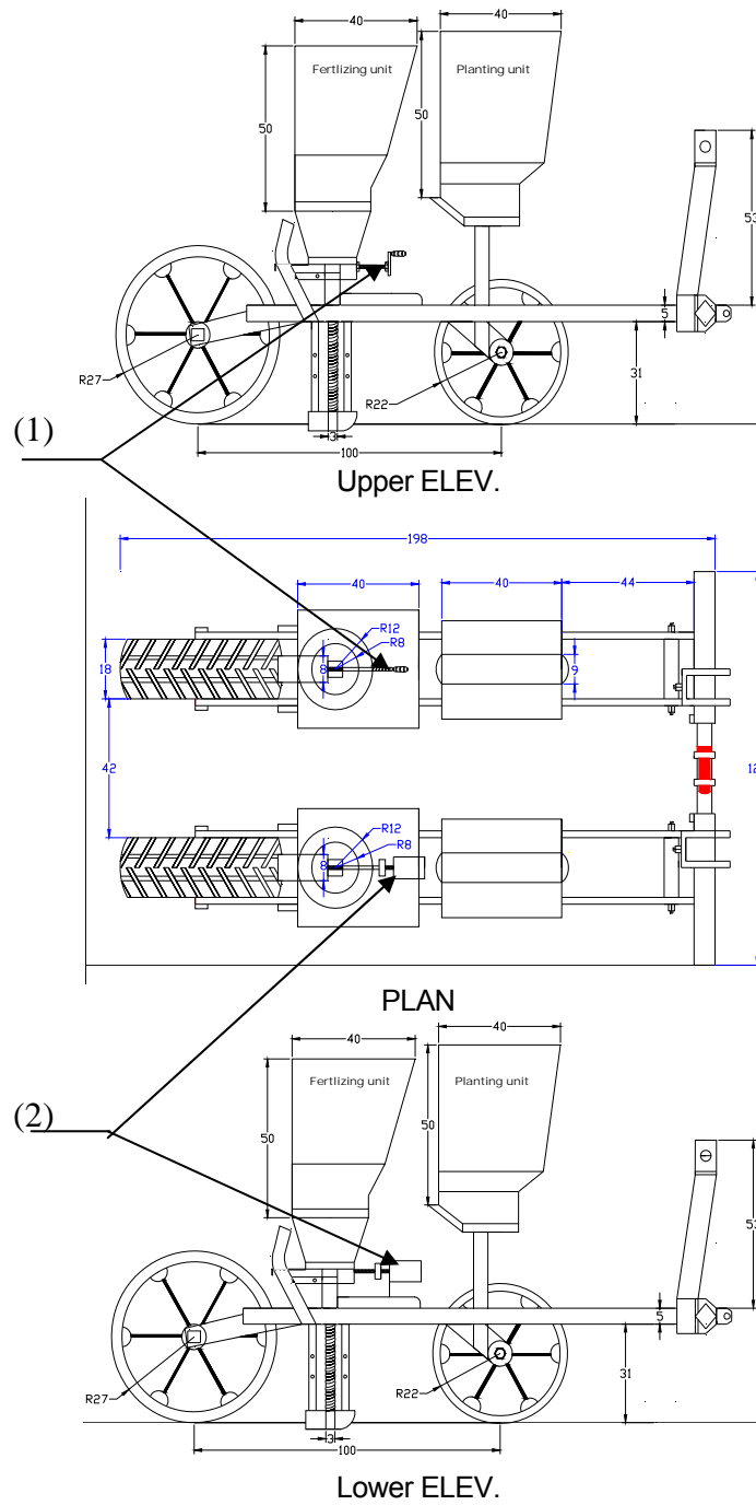
Fig. 1: A schematic drawing of the traditional and developed units.
