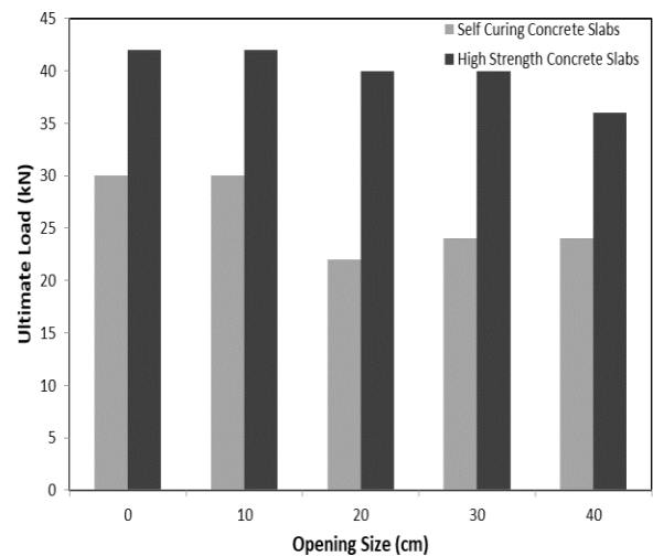
Fig.(17)Comparison between Self Curing Reinforced Concrete Slabs and High Strength Reinforced Concrete Slabs [7] at Ultimate Load with Different Opening Size
