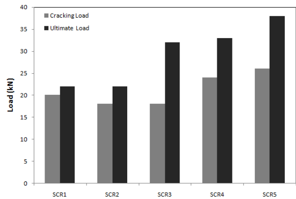
Fig. (10) Cracking and Ultimate Load for RC plates of Group (I) Effect of Reinforcement Ratio \mu\%
