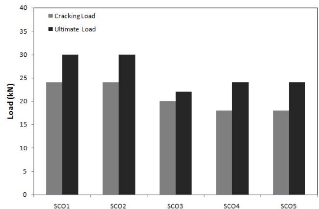
Fig. (11) Cracking and Ultimate Load for RC plates of Group (II) Effect of Opening Size
