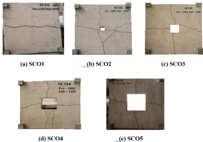
Figure (13) Mode of Failure for RSCC Group (II)
