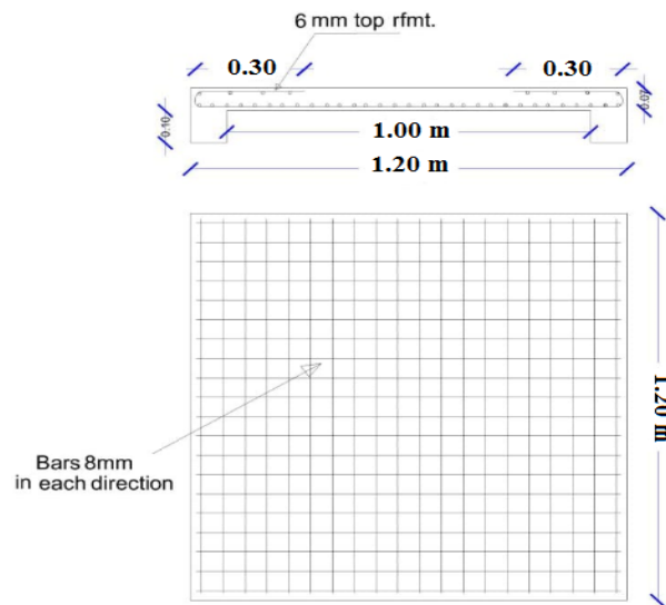
Fig.(3) Show dimensions of the typical tested slabs without opening and reinforcement details
