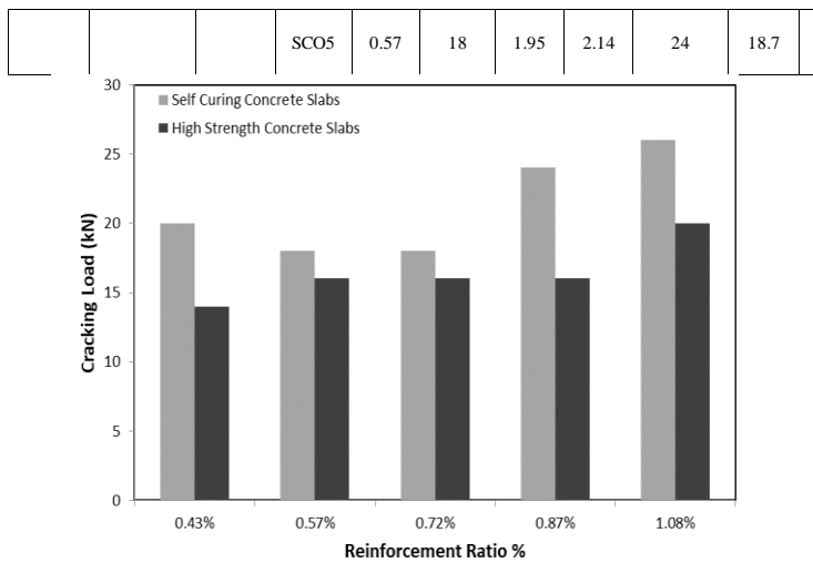
Fig.(14)Comparison between Self Curing Reinforced Concrete Slabs and High Strength Reinforced Concrete Slabs [7] at Cracking Load with Different Reinforcement Ratio \mu\%
