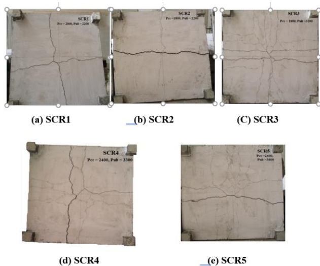
Figure (12) Mode of Failure for RSCC Group (I)
