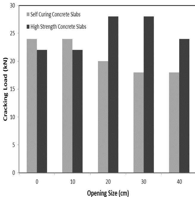
Fig.(15)Comparison between Self Curing Reinforced Concrete Slabs and High Strength Reinforced Concrete Slabs [7] at Cracking Load with Different Opening Size
