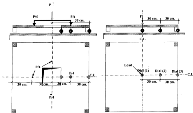
Fig. (5) Arrangement of Dials for Different Tested Plates [7]
