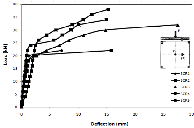
Fig. (7) Load -Deflection Comparison for RC Plates of Group (I) at Point (2)
