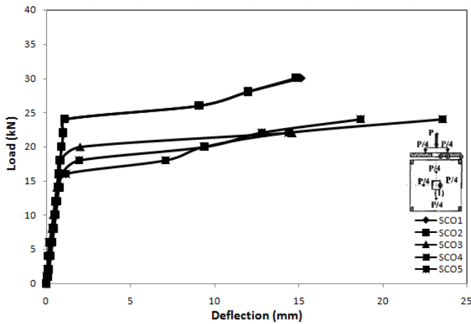
Fig. (8) Load -Deflection Comparison for RC Plates of Group (II) at Point (1)
