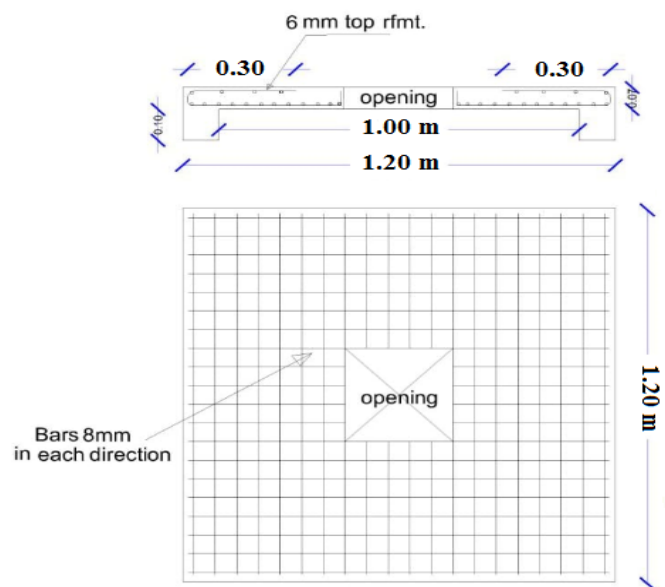
Fig. (4) Show dimensions of the typical tested slabs with opening and reinforcement details
