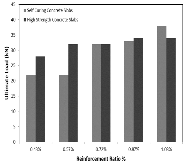
Fig.(16)Comparison between Self Curing Reinforced Concrete Slabs and High Strength Reinforced Concrete Slabs [7] at Ultimate Load with Different Reinforcement Ratio \mu\%
