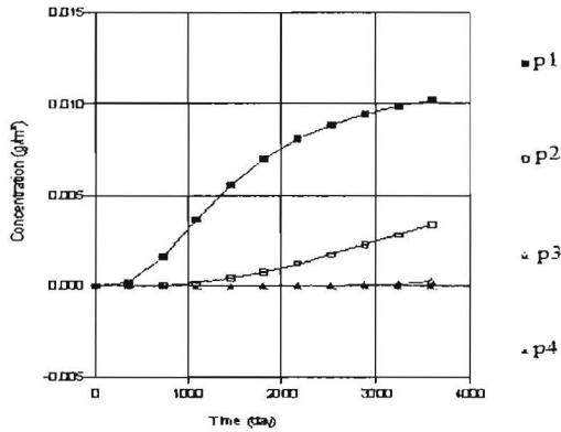
Fig. (7) Pb concentration with time at points (1, 2, 3, 4) at source concentration 0.05 gm/m^3 .
