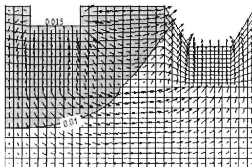
Fig. (4) Advection – dispersion analysis after (10years) for concentration (0.015 gm/m 3 ).
