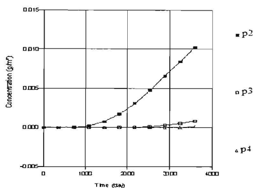
Fig. (22) Pb concentration with time at points (2, 3, 4).
