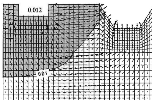
Fig. (5) Advection – dispersion analysis after (10years) for concentration (0.012gm/m 3 ).
