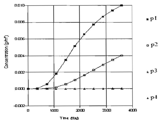
Fig. (16) Pb concentration with time at points (1, 2, 3, 4) at depth (2.0)m.
