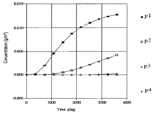
Fig. (9) Pb concentration with time at points (1, 2, 3, 4) at source concentration 0.015 gm/m^3 .
