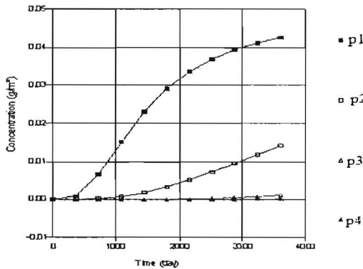
Fig. (8) Pb concentration with time at points (1, 2, 3, 4) at source concentration 0.03 gm/m^3 .
