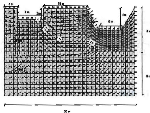
(1) Model Dimensions
