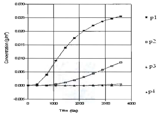
Fig. (10) Pb concentration with time at points (1, 2, 3, 4) at source concentration 0.012 gm/m^3 .
