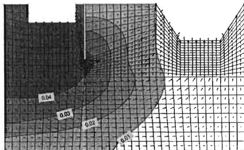
Fig. (14) Advection – dispersion analysis after (10 years) using sheet pile (6.0m) in depth.
