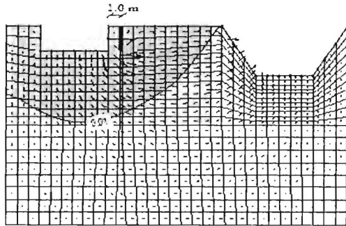
Fig. (11) Advection – dispersion analysis after (10 years) using sheet pile (2.0 m) in depth.
