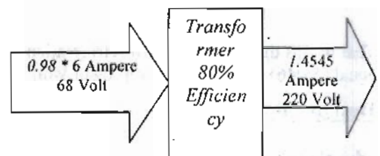
Fig 12: The transformer.
