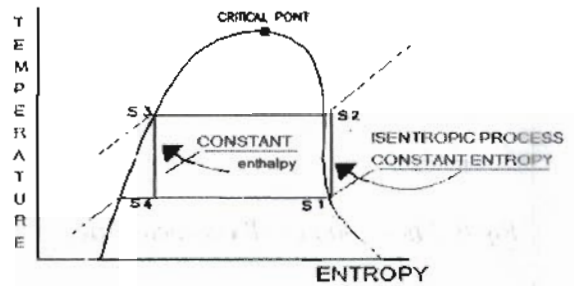
Fig 10b: T-S diagram for a refrigeration cycle
