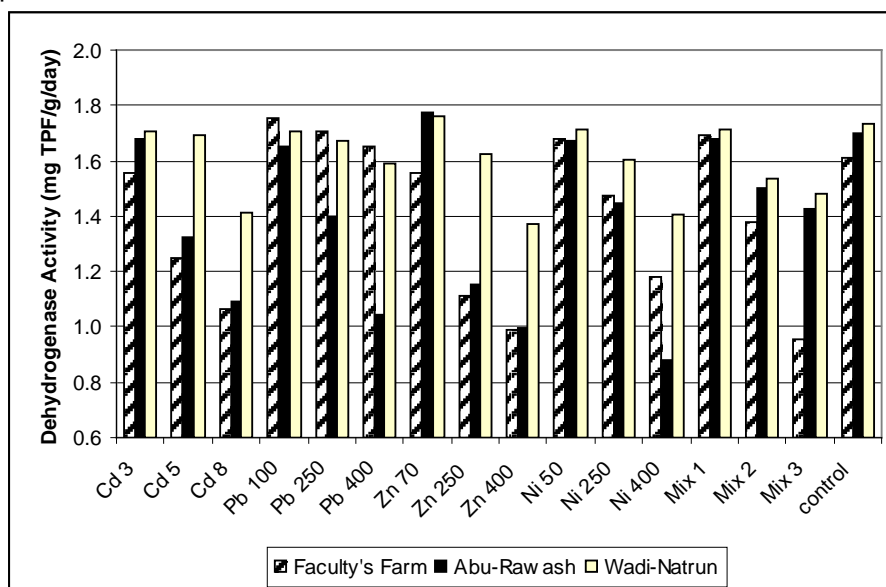
Fig. 2: Dehydrogenase activity of the three soil types as affected by increased applied rates of Cd, Pb, Zn and Ni.
