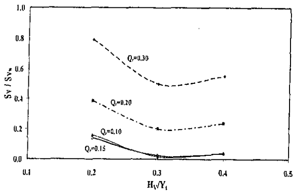
Figure (5) Relationship between H_v/Y_t , and S_V/S_{Vw} , for different Q_r
