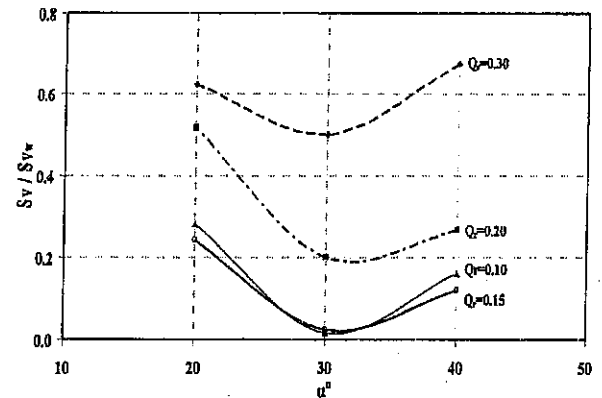
Figure (3) Relationship between \alpha , and S_v/S_{vw} , for different Q_r
