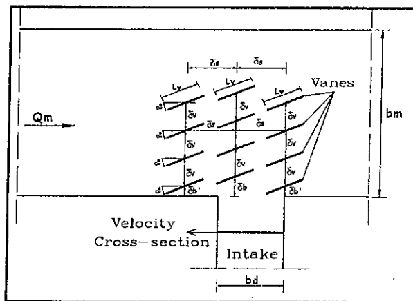
b- Layout of triple vane rows
