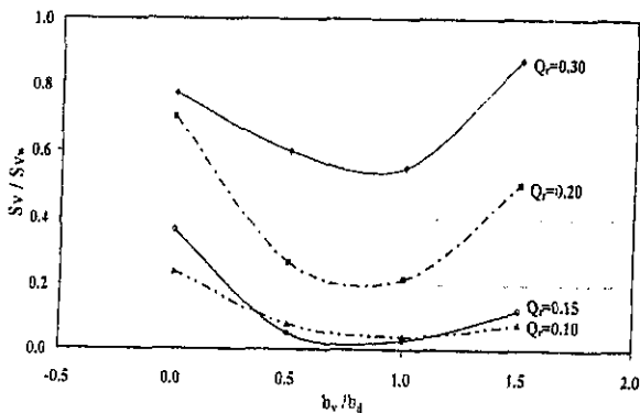
Figure (7) Relationship between b_v/b_d , and S_V/S_{Vw} , for different Q_r
