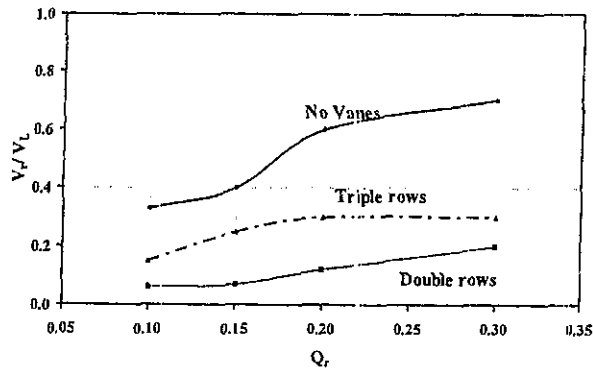
Figure (9) Relationship between Q_r , and v_r/v_L for different vane cases
