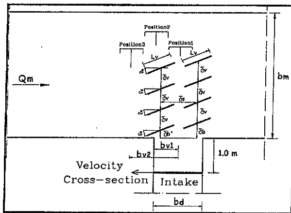
a- Layout of double vane rows
