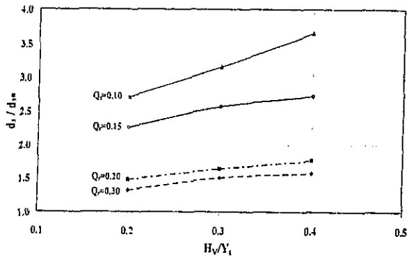
Figure (6) Relationship between H_v/Y_t , and d_s/d_{sw} , for different Q_r
