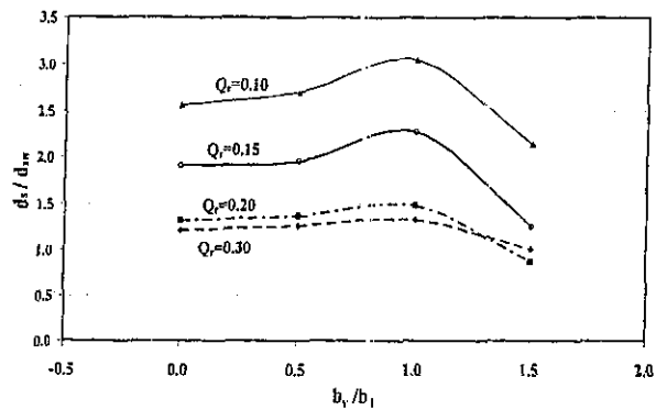
Figure (8) Relationship between b_v/b_d , and d_s/d_{sw} , for different Q_r
