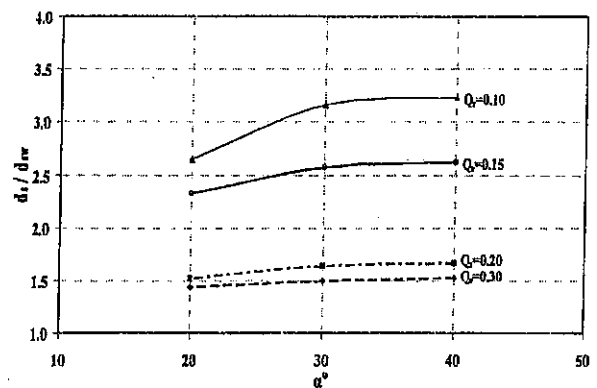
Figure (4) Relationship between \alpha , and d_s/d_{sw} , for different Q_r
