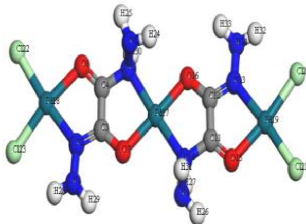
Fig.7. Structure of [\text{Pd}_3(\text{ODH2H})\text{Cl}_4](\text{H}_2\text{O})_2].2\text{C H}_3\text{OH}
