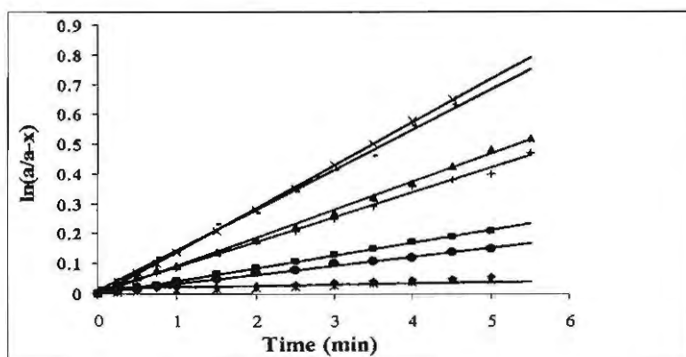
Fig. (5): First order relation \ln(a/a-x) = kt at 303 K: (x); S sulph * , (-); S sulph , (▲); S * , (+); S, (■); S TX * , (●); S TX , (◆); S CPB * and (□); S CPB
