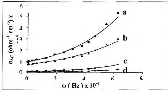
Fig. 4: The frequency dependence of AC-conductivity for: (a); S_{CPB} , (b); S_{TX} , (c); S , and (d); S_{Suloh}
