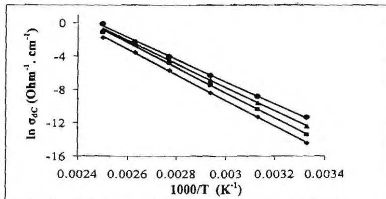
Fig. 3: The temperature dependence of DC-conductivity for: (●); S_{CPB} , (▲); S_{TX} , (■); S , and (◆); S_{(Sulph)}
