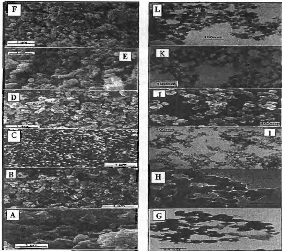
Fig. 2a: SEM of: A- S B- S_{sulph} C- S_{TX} D- S_{CPB} E- S^* and F- S^*_{TX} Fig. 2b: TEM of: G- S_{sulph} H- S I- S_{TX} J- S_{CPB} K- S_{CPB}^* and L- S^*
