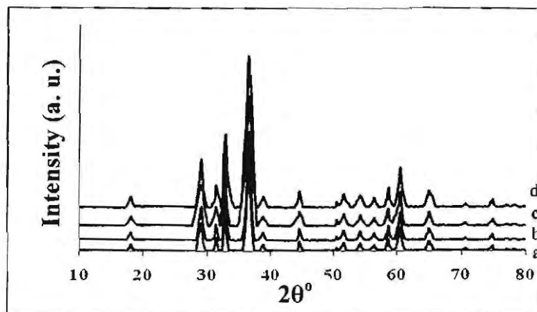
Fig. 1: X-ray diffraction patterns of : a- S_{sulph} b- S c- S_{TX} and d- S_{CPB}
