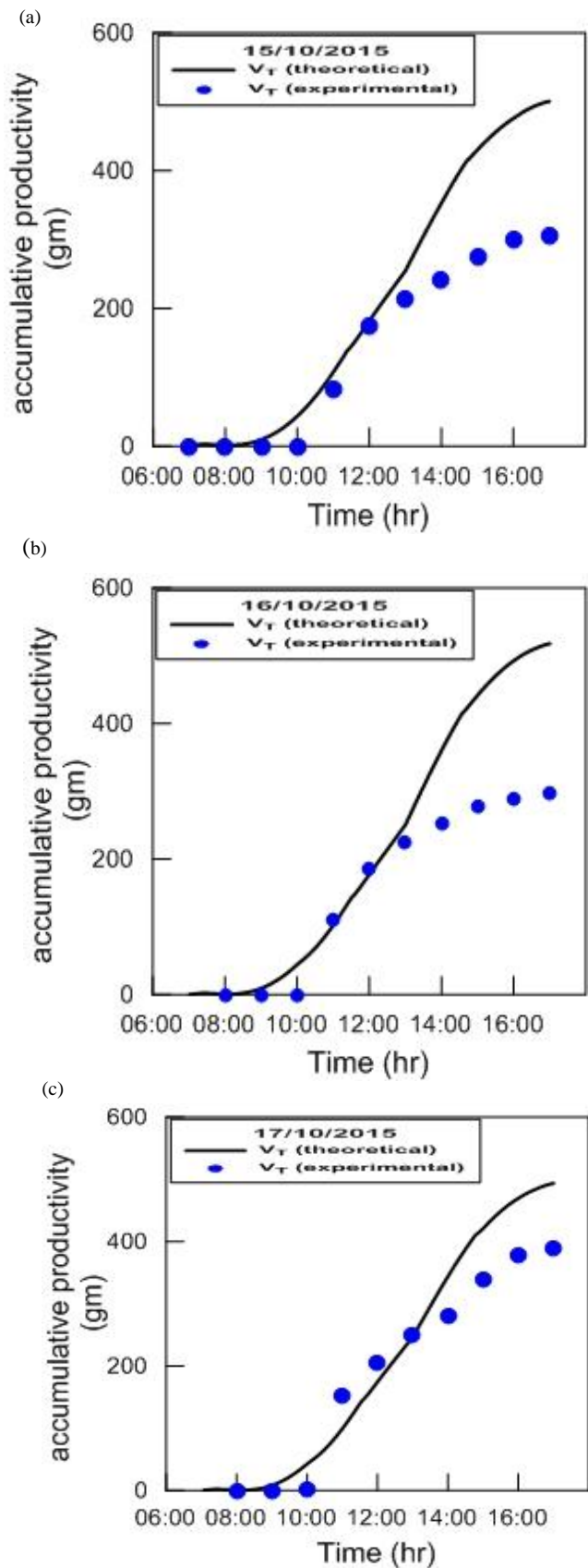
Fig .10. Comparison between theoretical and experimental productivity.
