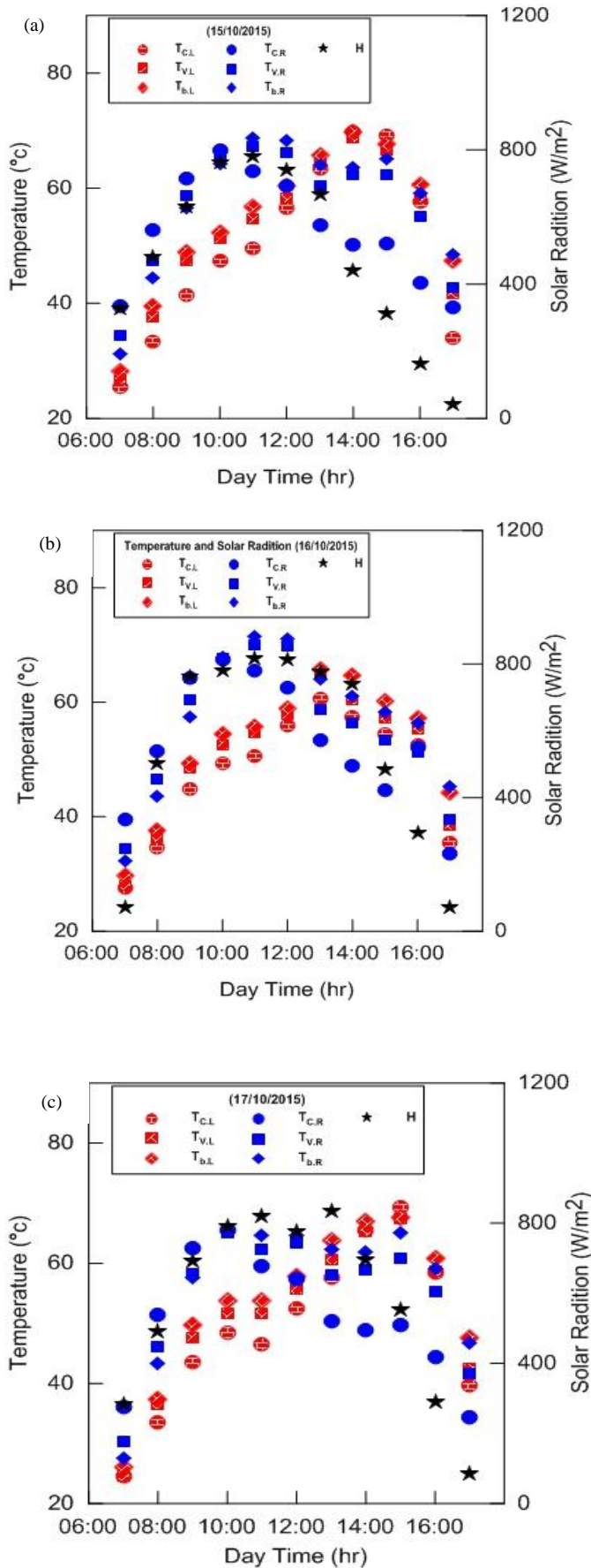
Fig.7. Experimental hourly temperature and solar radiation for the period (15-17/10/2015).
