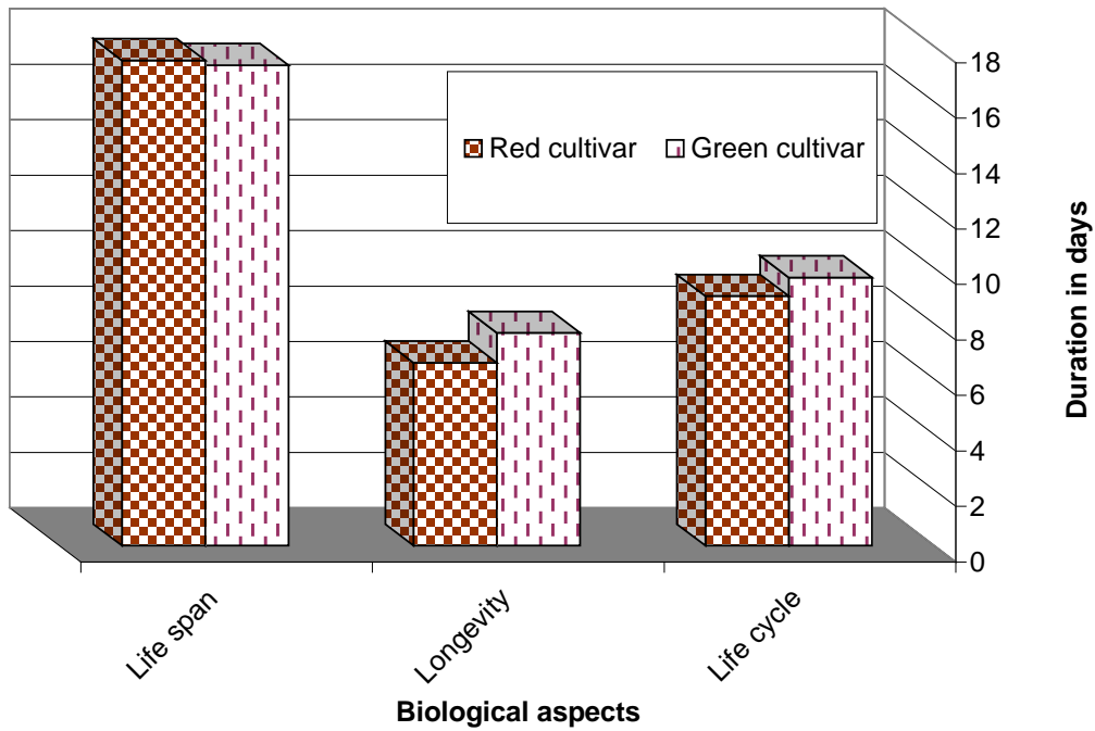
Fig. ( 1 ) : Duration of the two spotted spider mites, Tetranychus urticae adult females when fed on two castor cultivars.
