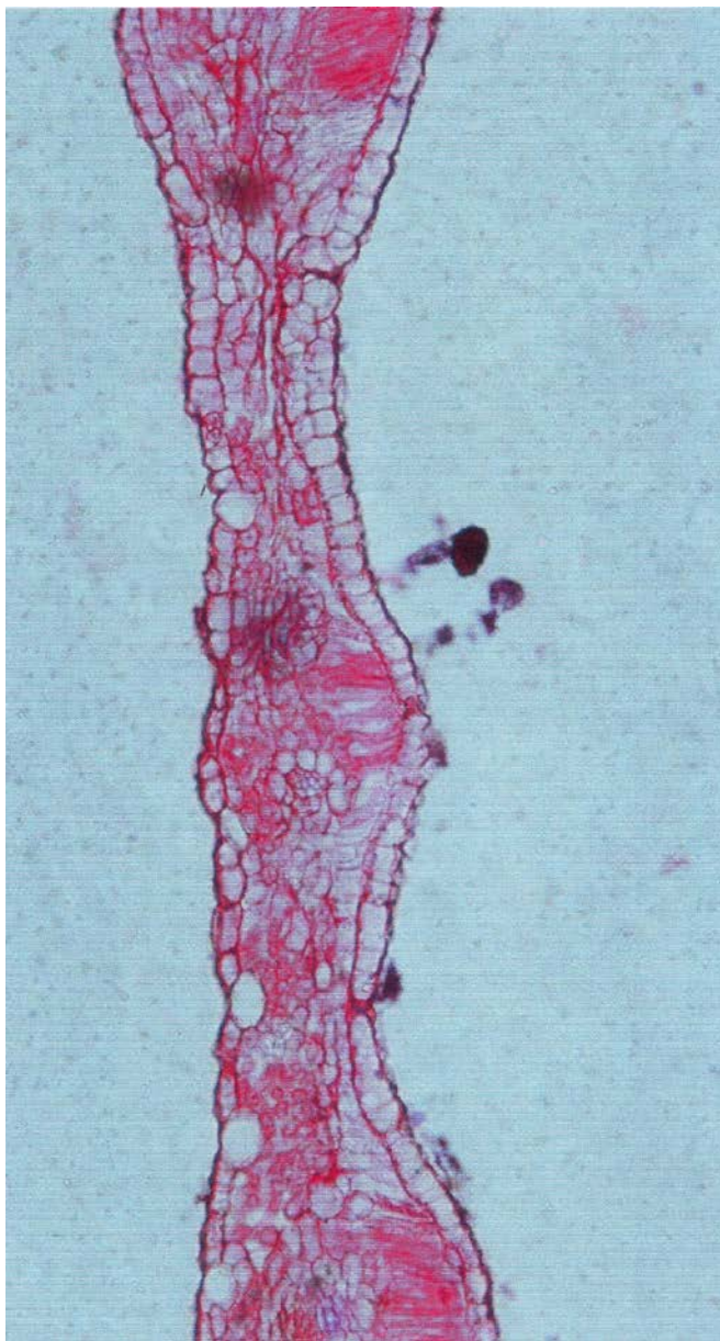
Fig. 5: Cross section through the middle part of leaf for green cultivar.
