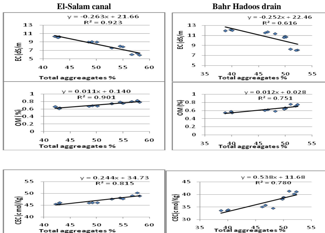
Fig. 2. Relationship between EC and total stable aggregates, O.M and total stable aggregates and CEC and total stable aggregates under different treatments in the studied soils.
