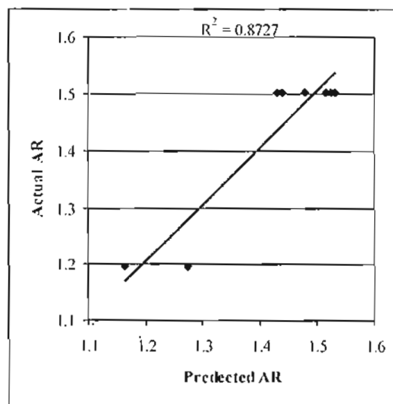
Fig. (3) Actual Accident Rates versus Predicted Accident Rates in "Straight Road Section in Unoccupied Areas"
