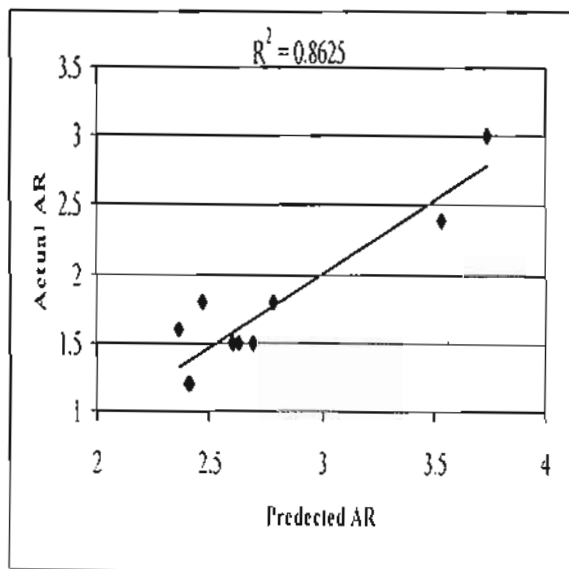
Fig. (4). Actual Accident Rates versus Predicted Accident Rates in "Curved Road Section in Agricultural or Residential Areas"
