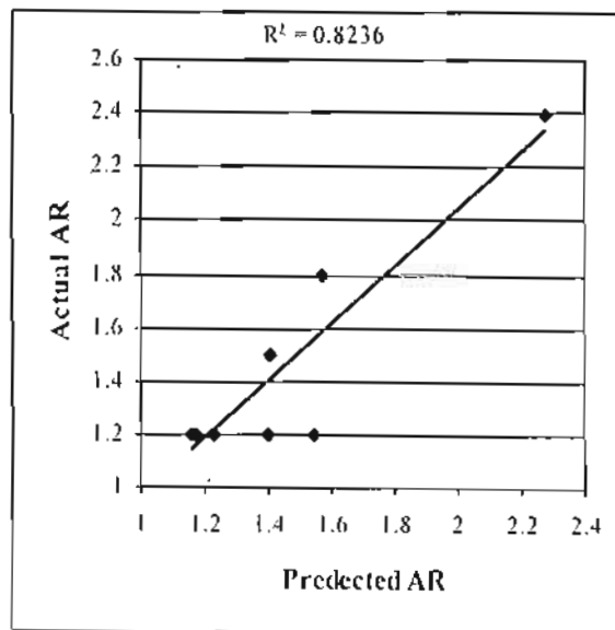
Fig. (5) Actual accident rates versus predicted accident rates in "curved road section in unoccupied areas"
