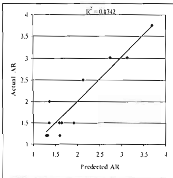
Fig. (2) Actual Accident Rates versus Predicted Accident Rates in "Straight Road Section in Agricultural or Residential Areas"
